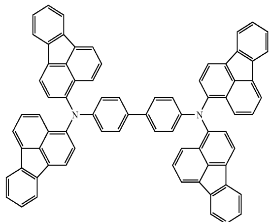
Structural Formula (F7)
