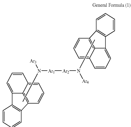
General Formula (1)
