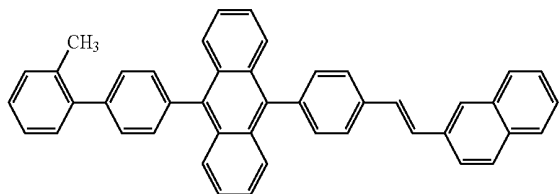
Structural Formula (A5)
