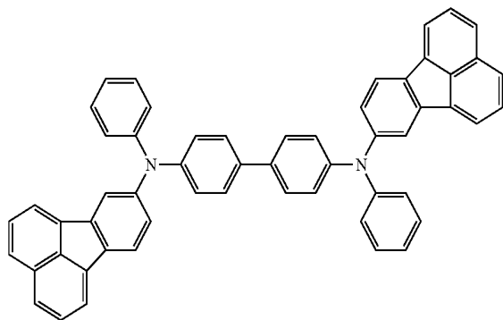
Structural Formula (F21)
