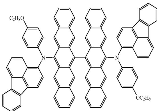
Structural Formula (F20)
