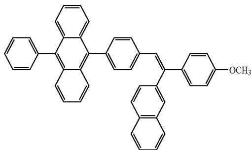
Structural Formula (A7)
