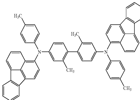
Structural Formula (F10)
