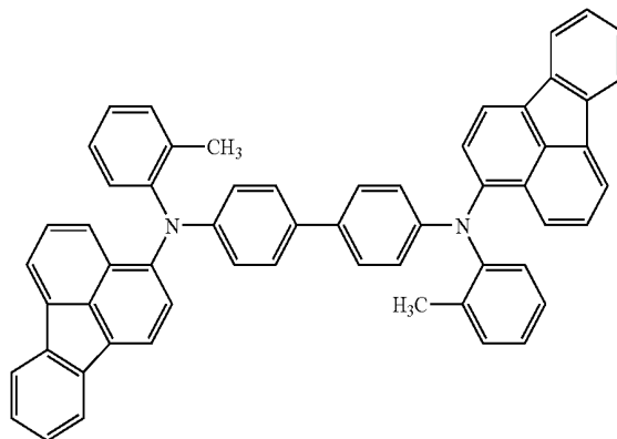
Structural Formula (F3)
