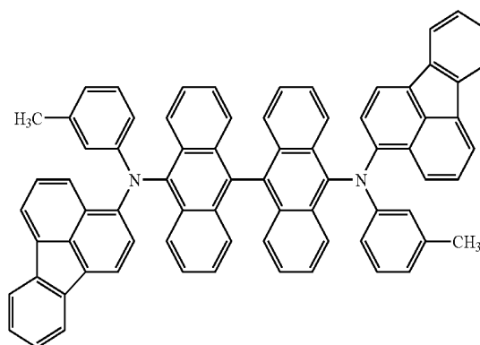
Structural Formula (F15)
