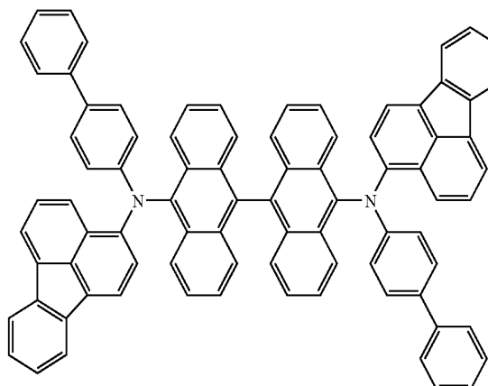
Structural Formula (F18)
