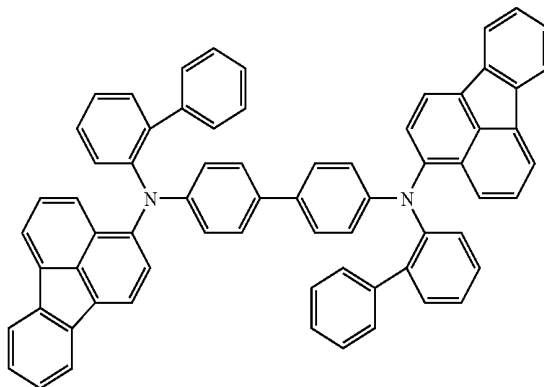
Structural Formula (F9)
