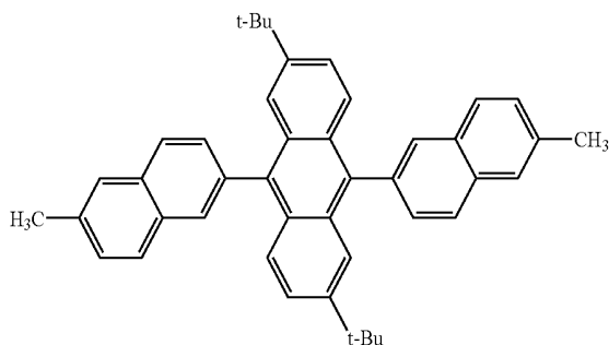
Structural Formula (A4)
