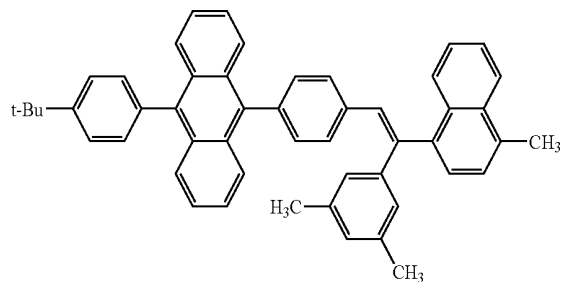
Structural Formula (A5)
