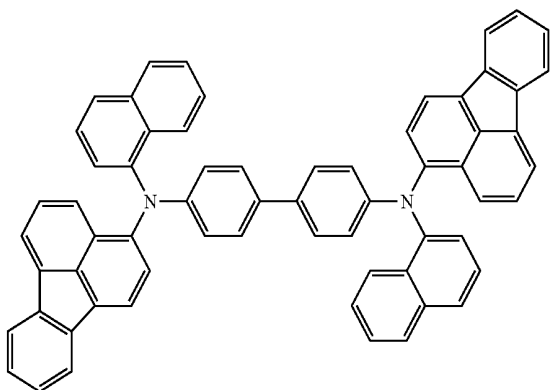
Structural Formula (F5)
