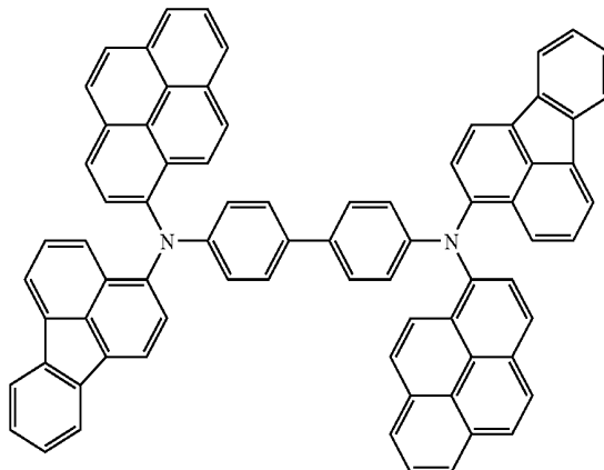
Structural Formula (F9)
