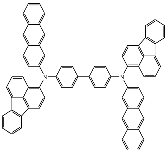
Structural Formula (F6)
