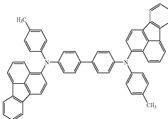
Structural Formula (F4)
